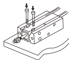
Side-connected (with through bore in the body)
