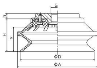
SZB75...150□-G3M
