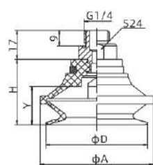
SZB50□-G2M
