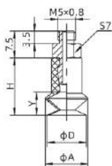
SZB5□-M5M SZB8...15□-M5M
