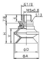
SZB17...20□-G1M
