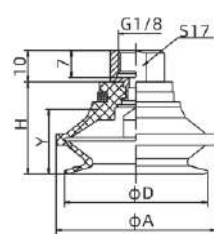
SZB30...40□-G1F
