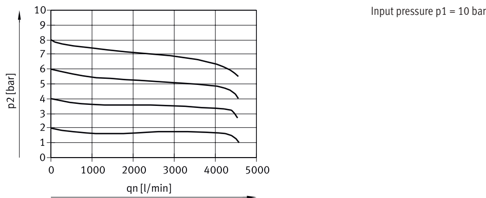
Standard flow rate qn as a function of output pressure p2 (LFR/LFRS-1/2-D-MIDI)
