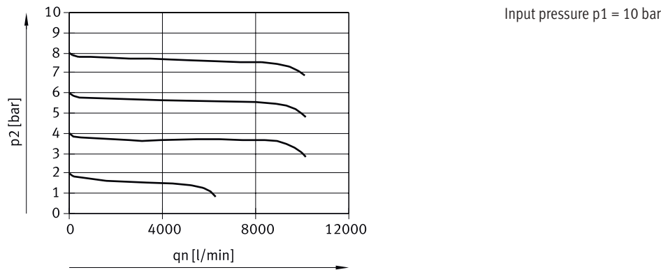
Standard flow rate qn as a function of output pressure p2 (LFR/LFRS-1-D-MAXI)
