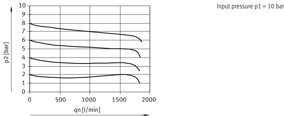
Standard flow rate qn as a function of output pressure p2 (LFR/LFRS-1/4-D-MINI)
