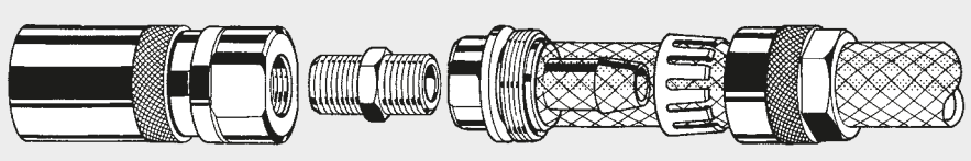
Female body plus self-locking hose fitting patented by Metal Work. When the outer ring nut is tightened, the gripper locks on the pipe.
