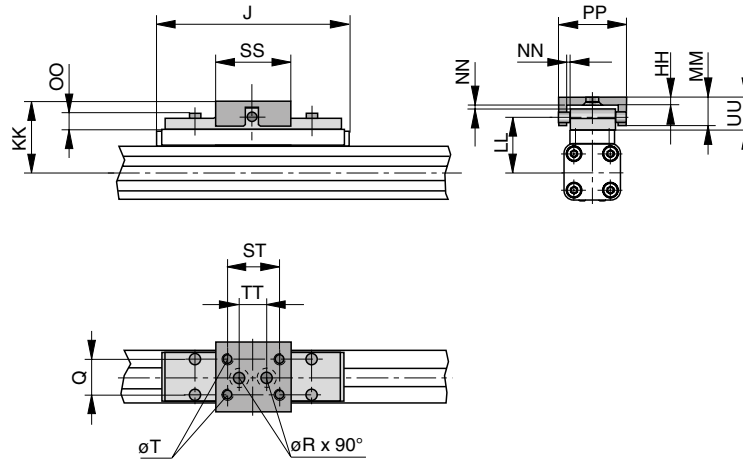
Series OSP-P16 to 50
