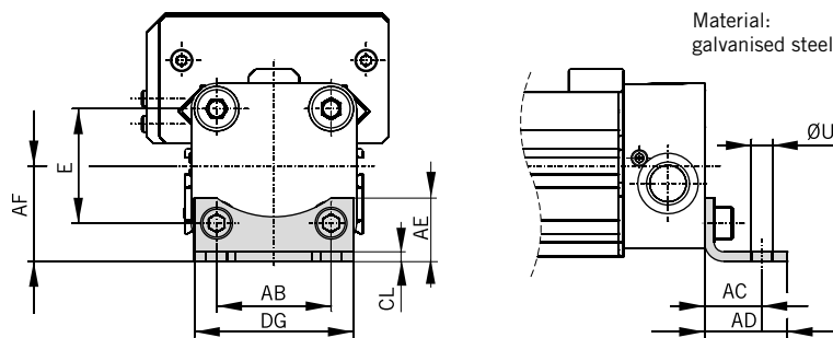
Series OSPP-BG40 and BG50: Type C1
