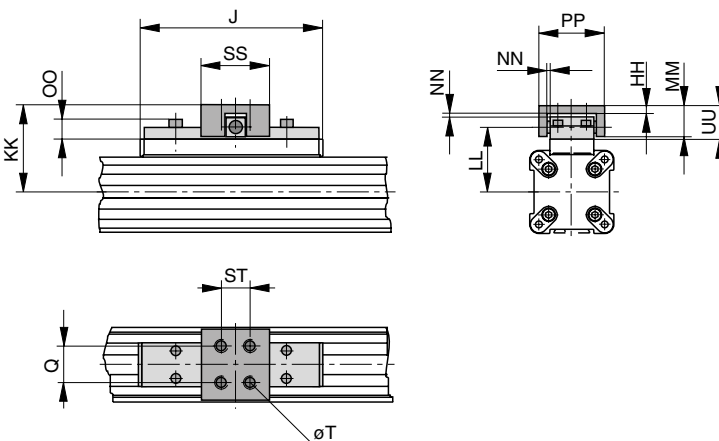
Series OSP-P63 and 80
