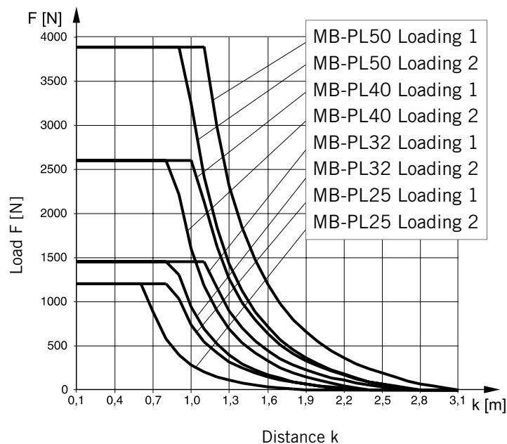
Permissible Unsupported Length OSP-P MB-PL25, MB-PL32, MB-PL40, MB-PL50
