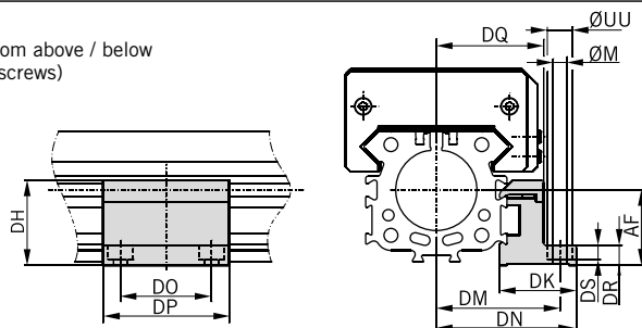
Series OSPP-BG25 to BG50: Type D1BG
