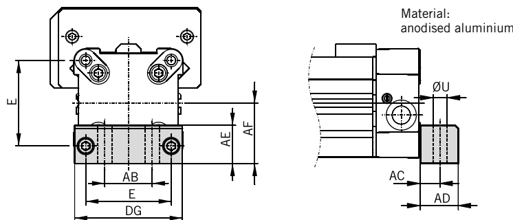
Series OSPP-BG25 to BG50: Type E1BG
