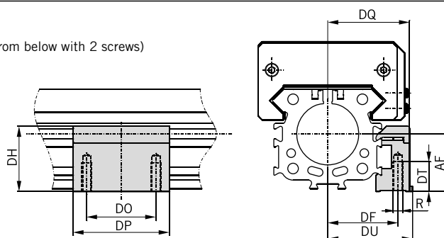
Series OSPP-BG25 to BG50: Type D1BG
