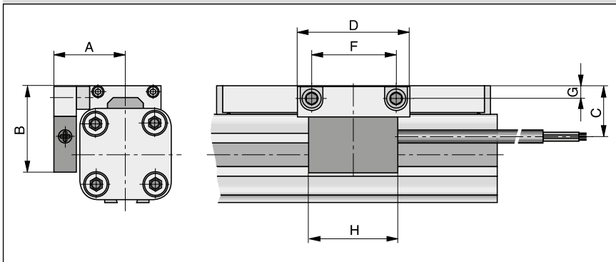
Dimension Table [mm]
