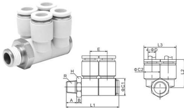
KQ2ZD 系列-2个双管万向弯头 KQ2ZD Series
