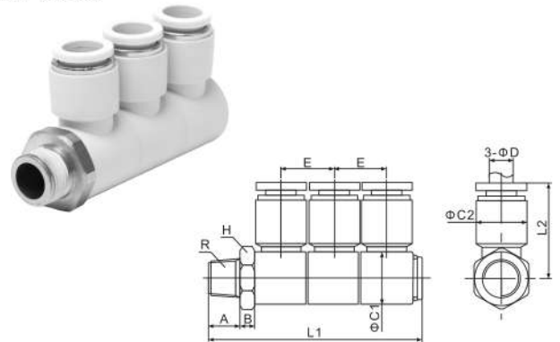
KQ2VT 系列-3个单管万向弯头 KQ2VT Series
